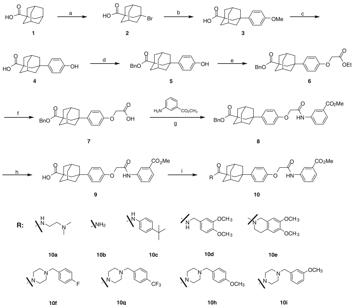
Scheme 1. Reagents and conditions: (a) AlCl 3 , Br 2 , –5 °C to rt, 93%; (b) anisole, AlCl 3 , –10 °C to rt, 94%; (c) BBr 3 , –10 °C to rt, 84%; (d) BnBr, KHCO 3 , 40 °C, 85%; (e) ethylchloroacetate, K 2 CO 3 , rt, 85%; (f) LiOH, THF/H 2 O, 97%; (g) PyBOP, DMAP, rt, 72%; (h) H 2 , Pd/C, 94%; (i) EDC, DIPEA, HOBt, rt, 55% for 10a or PyBOP, DMAP, rt, 94% for 10b ; or PPAA, Et 3 N, DCM, rt for 10c-i (28–70%).
