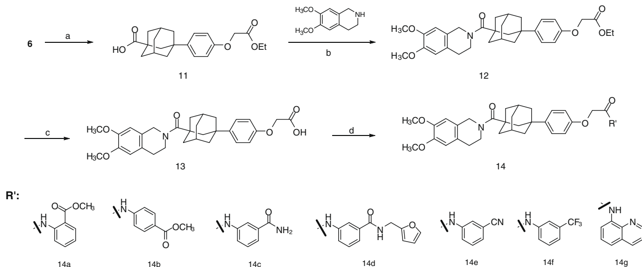
Scheme 2. Reagents and conditions: (a) Pd/C, MeOH, 99%; (b) PPA, Et 3 N, NaCN, rt, 66%; (c) LiOH, THF/H 2 O, 97%; (d) PPA, Et 3 N, NaCN, rt for 14a–c (32–40%) and 14e–f (42–50%); or (i) PPA, Et 3 N, NaCN, methyl 3-amino benzoate, rt, (ii) LiOH, THF/H 2 O, rt, (iii) EDC, DIPEA, HOBT, furfurylamine, rt for 14d (76%).
