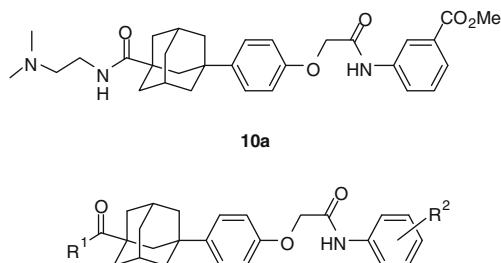
Figure 1. Hit molecule 10a identified from HTS and the general structure of the MDR revertants prepared in this Letter.
