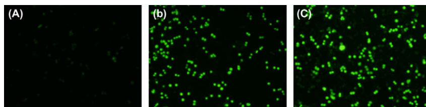
Figure 2. Inhibition of DiOC 2 efflux from MES-SA/DX5 cells by an adamantyl derivative 10h . The cells were treated with fluorescent P-gp substrate DiOC 2 , incubated for 1 h and washed three times with PBS. (A) Control, (B) 5 μM verapamil, (C) 1 μM 10h .
